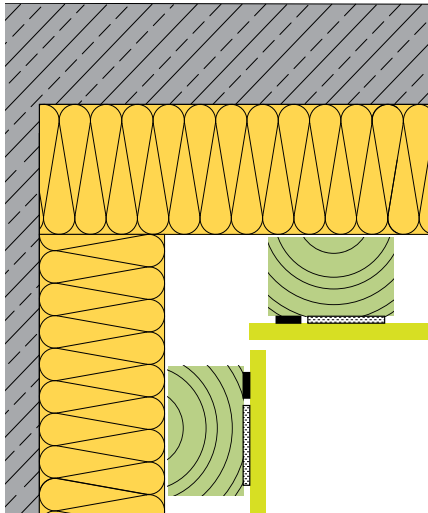
Binnenhoek A106
